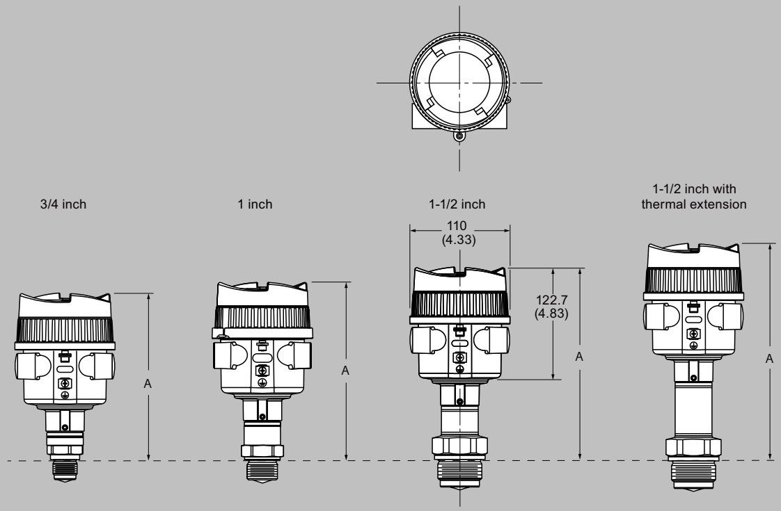
SITRANS LR510 Threaded lens antenna, dimensions in mm (inch)
